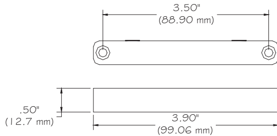
MAGNET
