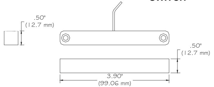
SWITCH
